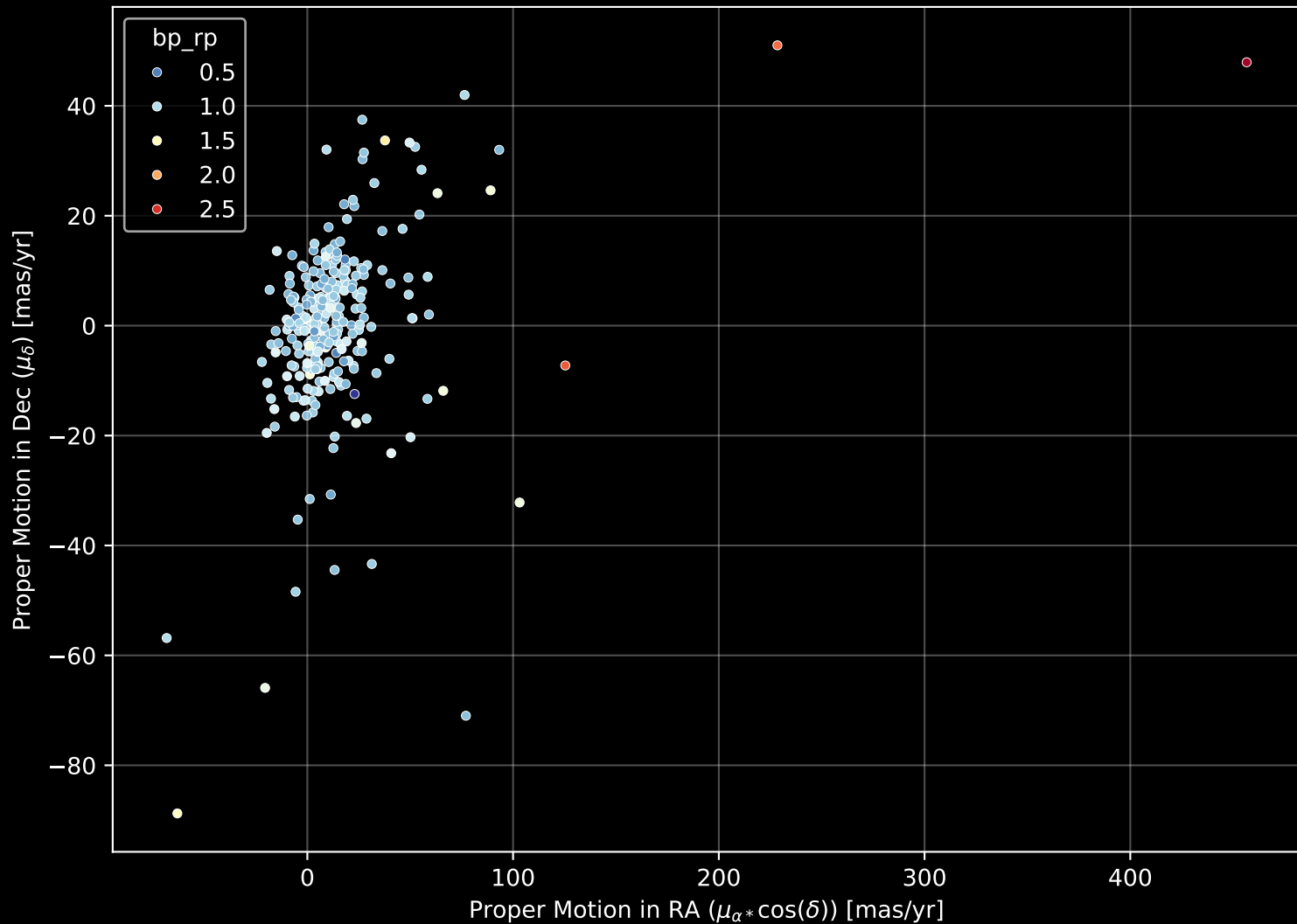
GALAH DR4 Field: [142] Proper Motion Diagram (n= 272)
