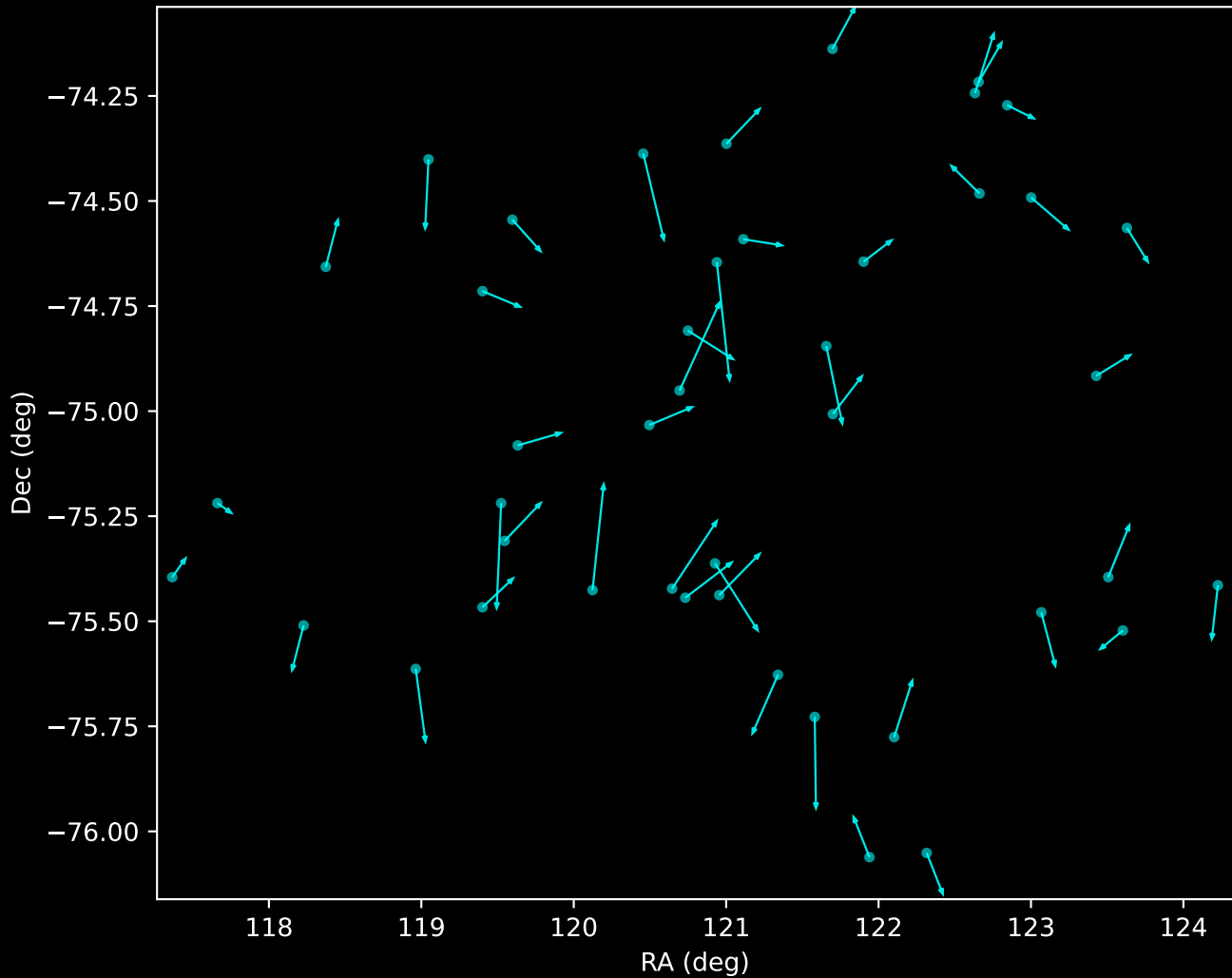
GALAH DR4 Noise Stream Proper Motion Vectors (n=44)
