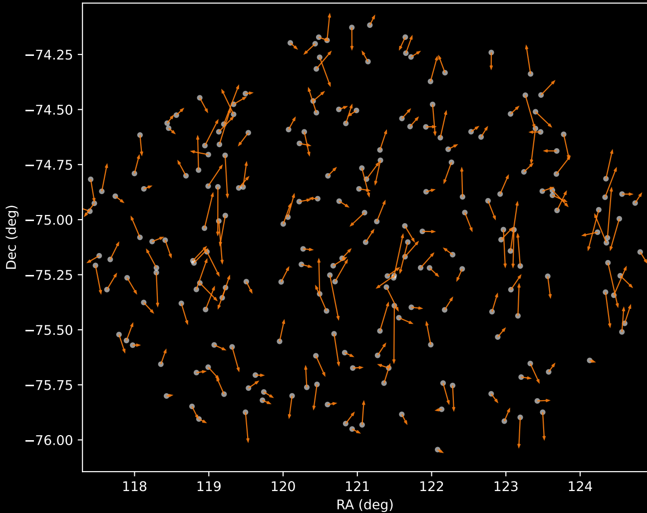
GALAH DR4 Cluster 2 Proper Motion Vectors (n=217)
